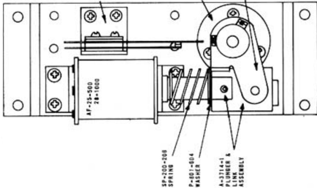
AS-1587-88 FLIPPER UNIT (LEFT) (AS SHOWN)
